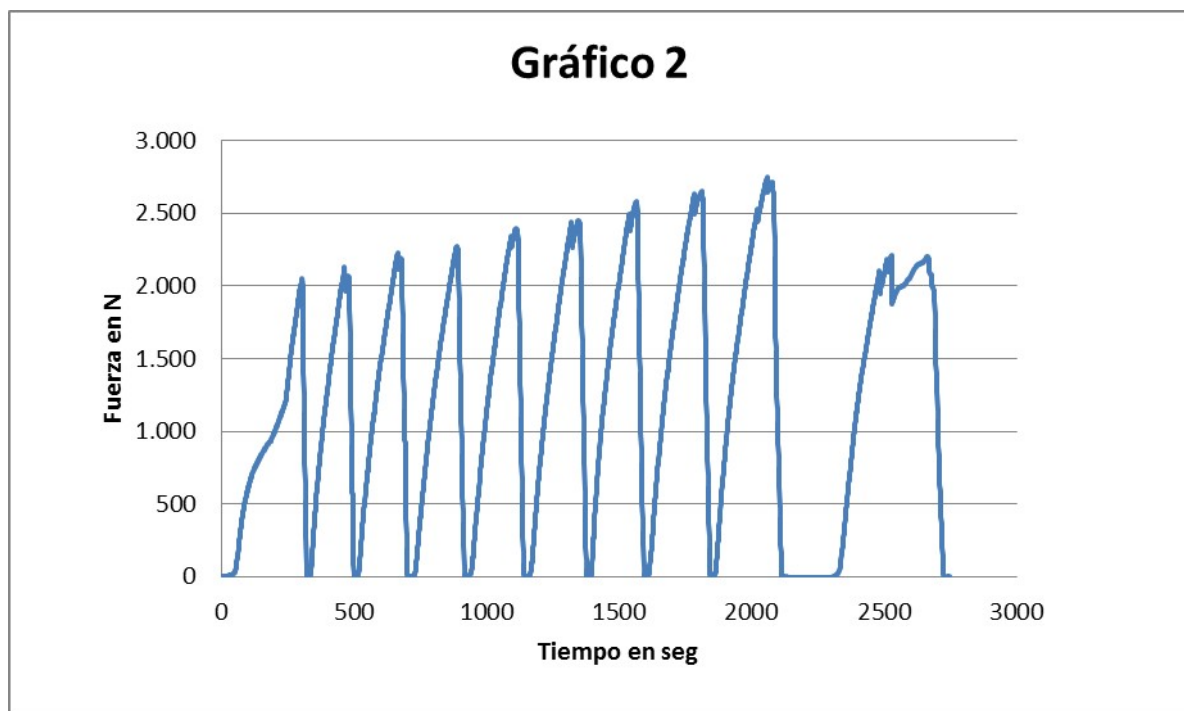
Graph 2: Load – Time in test 2
